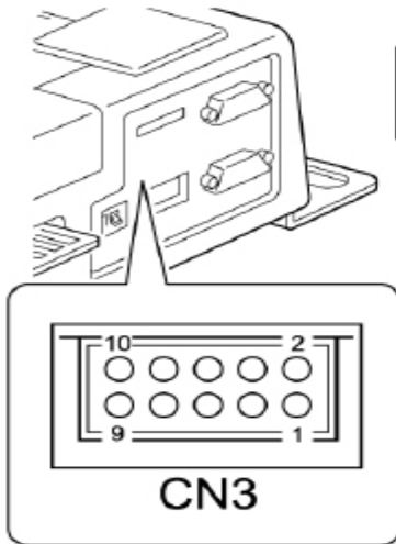
STEREO SPEAKER OUTPUT & EXTENSION SERIAL CONNECTOR, PIN LAYOUT (JST, 10 PIN PHD CONNECTOR)
