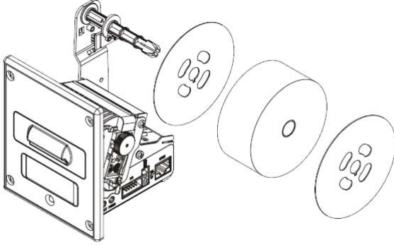
PRINTER WITH PAPER HOLDER Part#: 99-00-919
